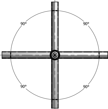
VIEW A-A SB-49 TOP VIEW DETAIL
